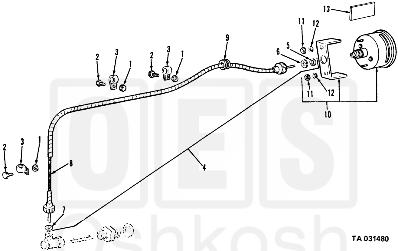
Figure 344. Tachometer.
